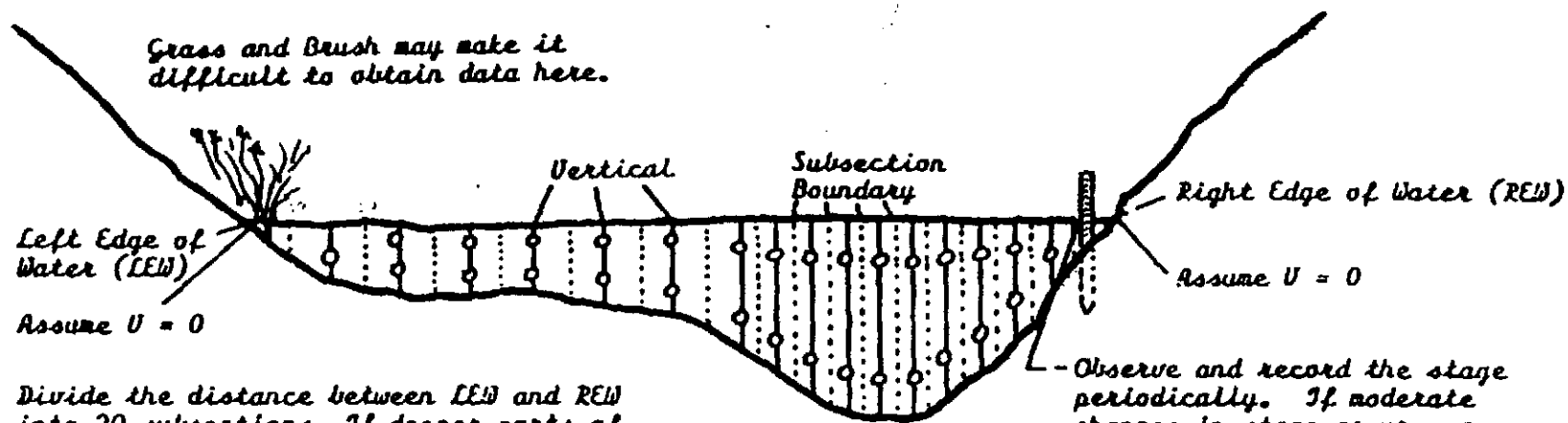
FIG. Measuring Stream Discharge in a Typical Cross Section (from Schulz 1978)
