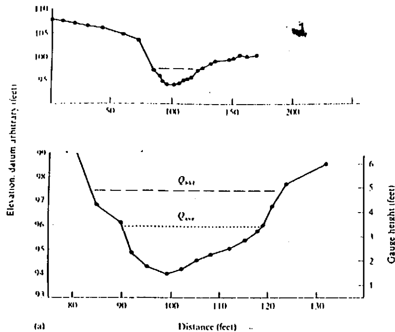
Figure 16-7 (a) New Fork River below New Fork Lake: drainage area 36.2 sq mi; slope .0051; bed material D_{50} 52 mm; Q_{15} 355 cfs; Q_{bank} 340 cfs; Q_{ave} 50.5 cfs. (b) Fall Creek near Pinedale, Wyoming: drainage area 37.2 sq mi; slope .040; bed material D_{50} 210 mm; Q_{15} 350 cfs; Q_{bank} 315 cfs; Q_{ave} 39.4 cfs. (c) Silver Creek near Big Sandy, Wyoming: drainage area 45.4 sq mi; slope .004; bed material D_{50} 45 mm; Q_{15} 600 cfs; Q_{bank} 390 cfs; Q_{ave} 43 cfs.
