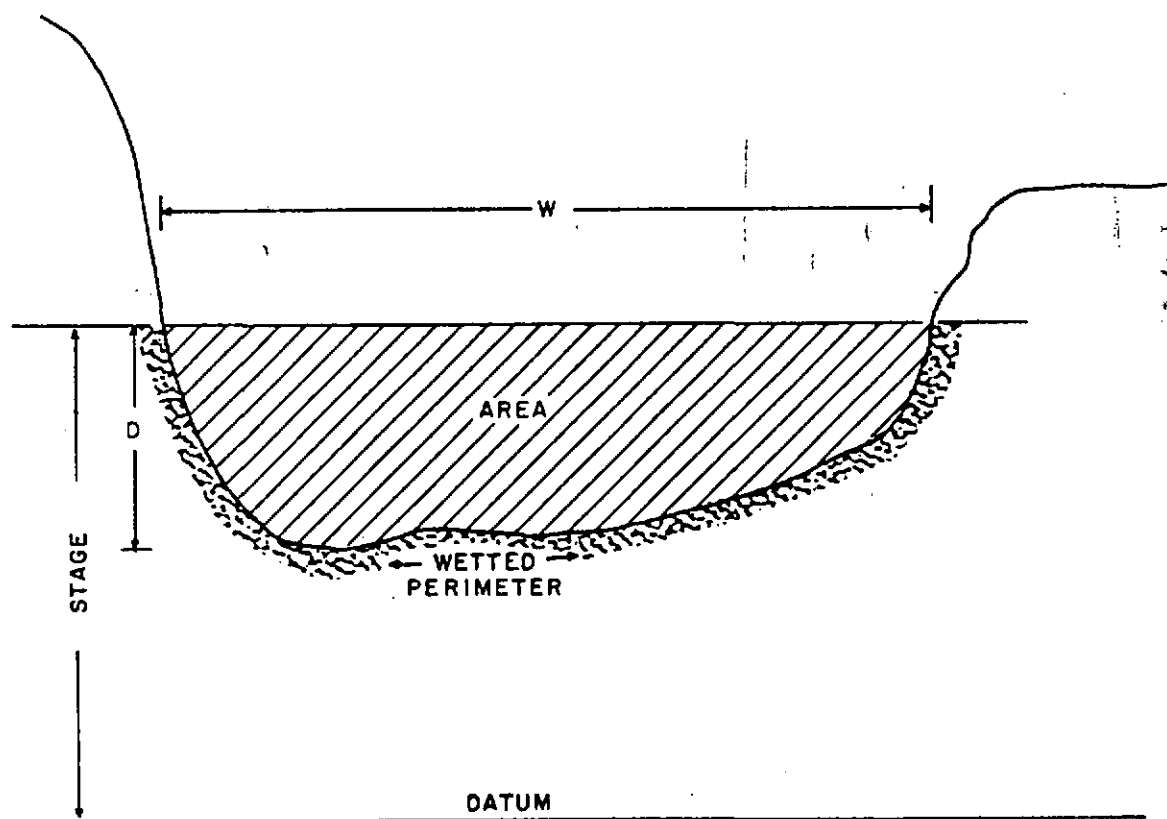
Fig. 4.1. Cross-sectional area of channel is computed as width ( W ) \times mean depth of the cross section. Stage is the elevation of the water surface above a datum (plane of known arbitrary elevation) (from Bovee and Milhous 1978).
