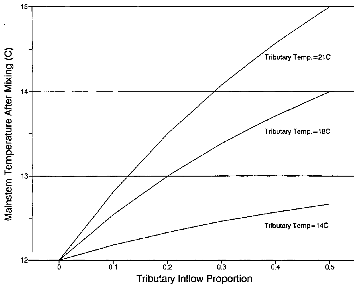
Figure 4. Temperature effects of tributary mixing. The mainstream temperature upstream of the confluence is assumed to be 12 degrees celcius. The influence on the downstream temperature is shown for incoming tributaries of three different temperatures.
